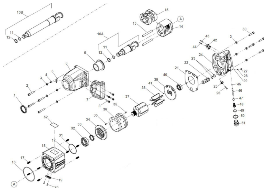
Figure 2: PT2500 & PT2500L Pneumatic Impact Wrench
