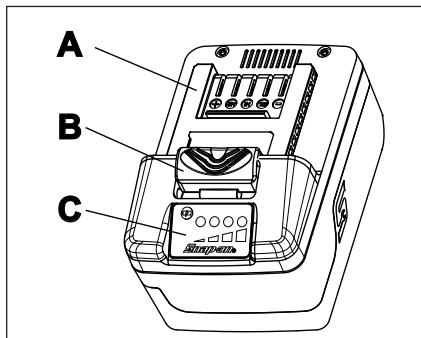
Figure 7 : Bloc-batterie (CTB8187)
