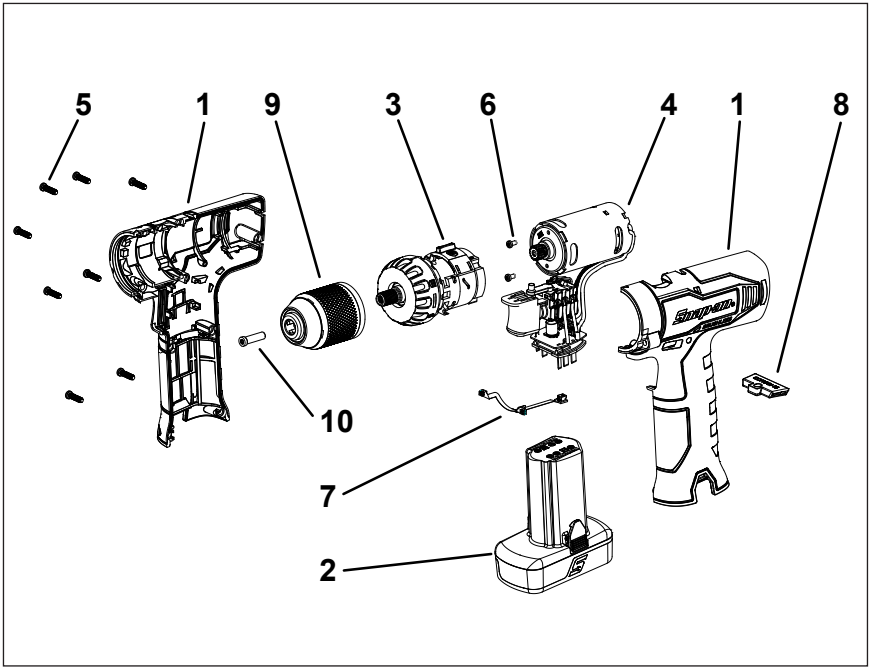
Figure 9: Exploded View
