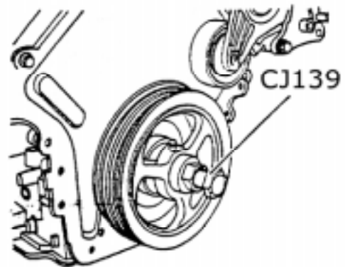
Installing Harmonic Balancer
